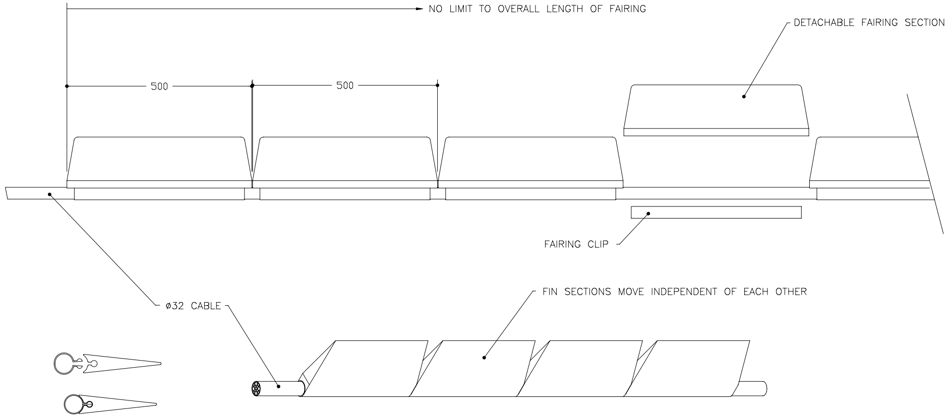
FAIRING CROSS SECTION
